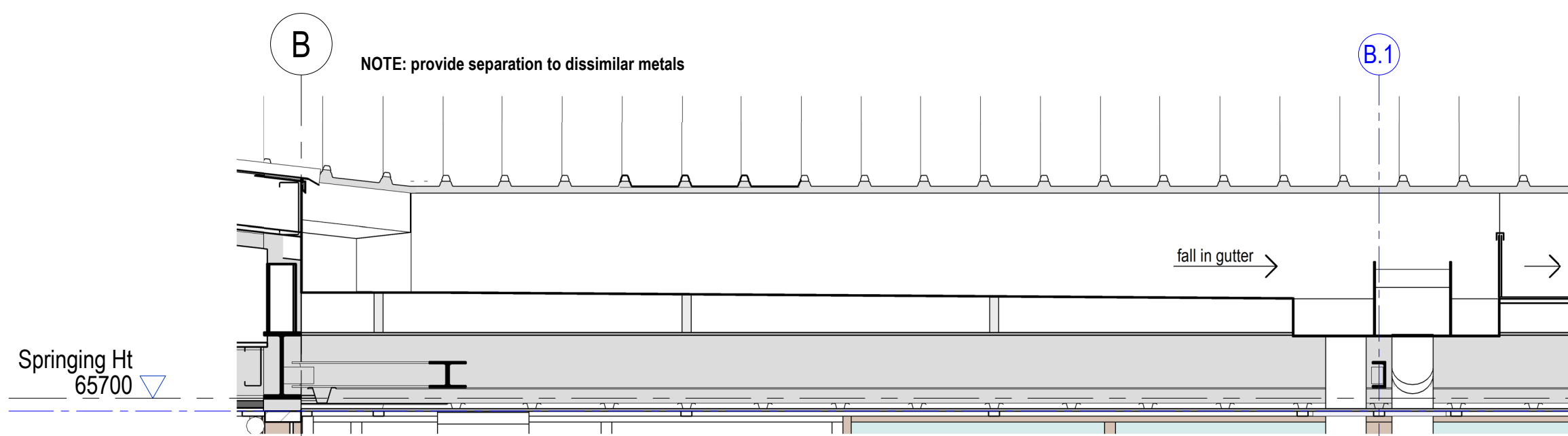
7 Valley Gutter to Sump 1:20
