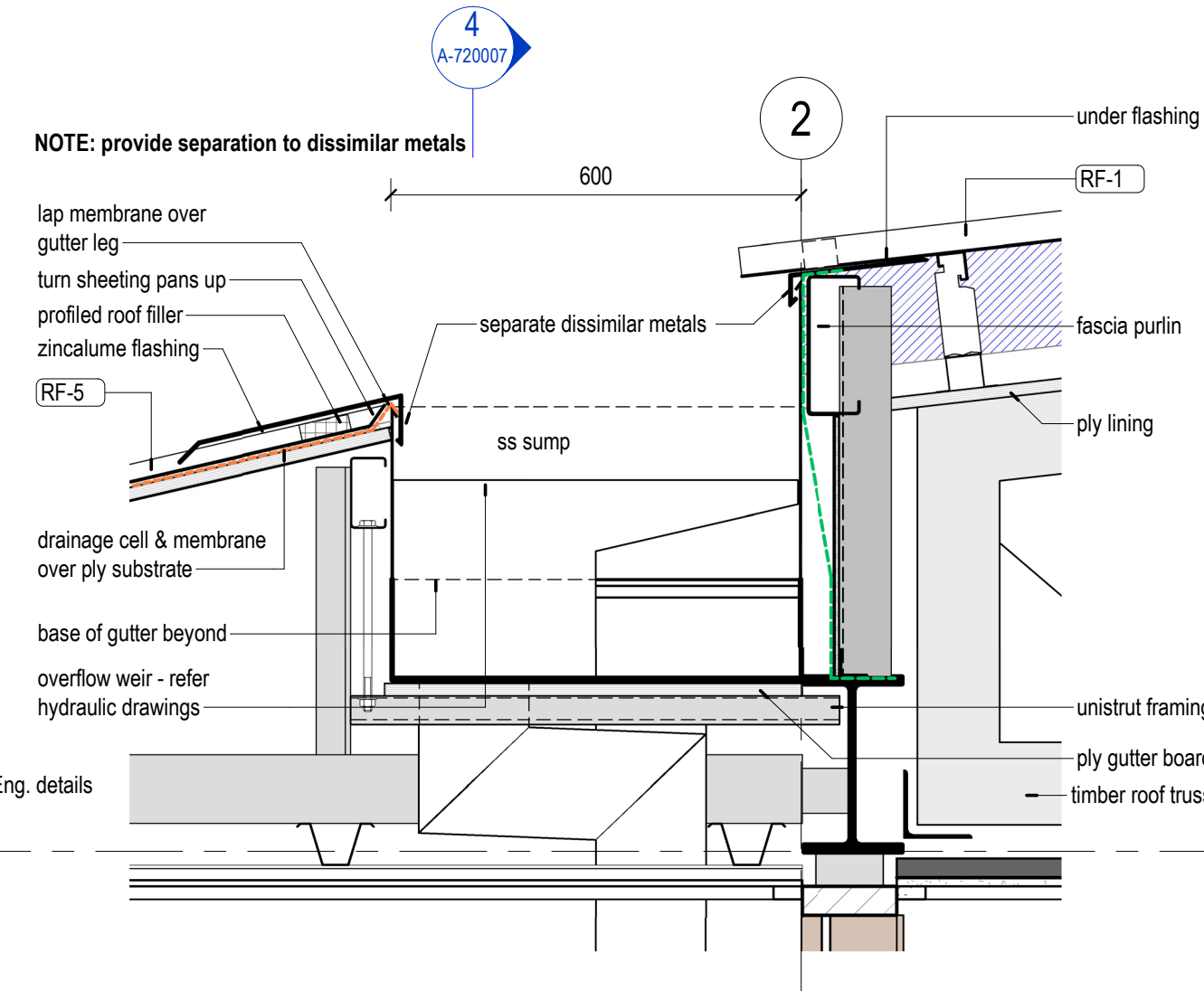
3 RG-1 Box Gutter Sump Section 1:10
