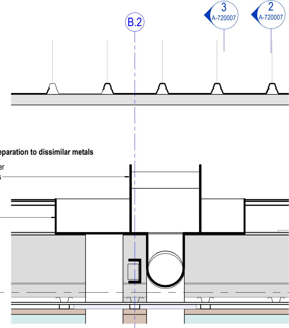
4 RG-1 Box Gutter Sump Long Section 1:10
