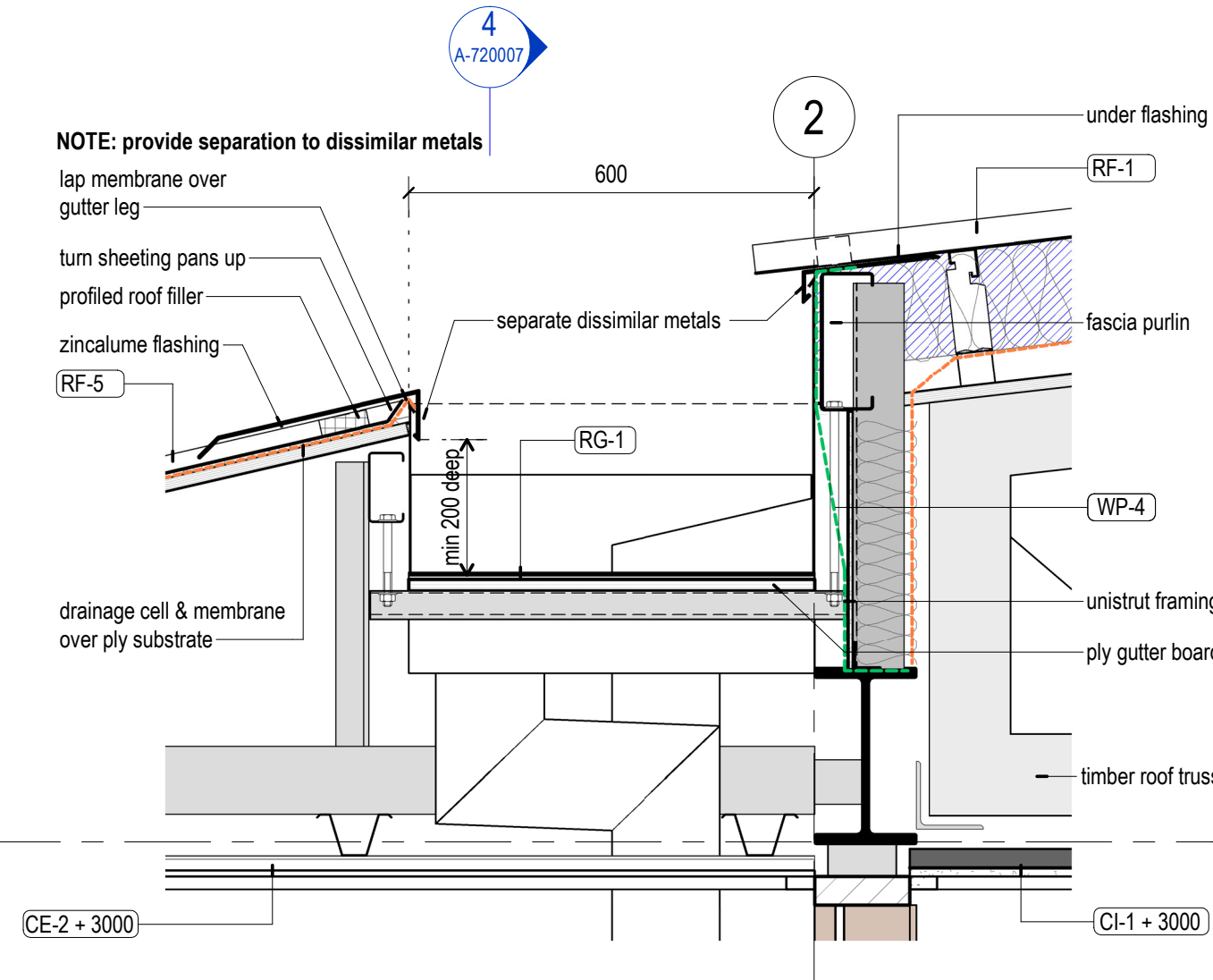
2 RG-1 Box Gutter Section 1:10
