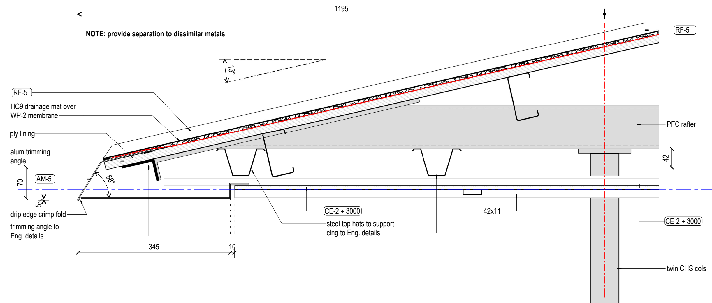
6 Courtyard North + West Facade Section 1:5
