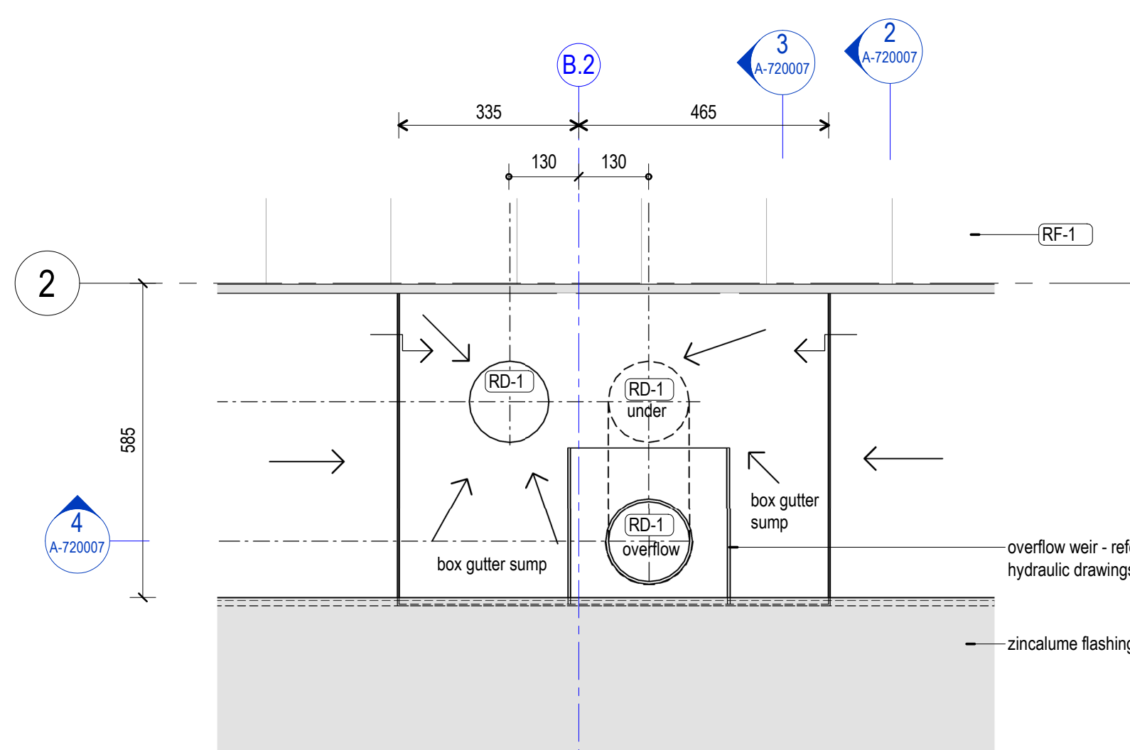
1 RG-1 Box Gutter Sump Plan 1:10
