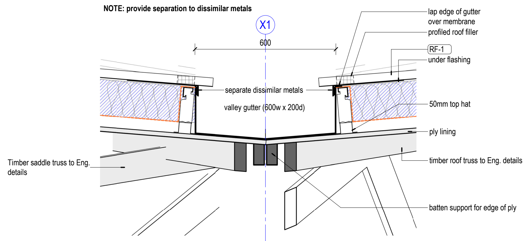
5 Valley Gutter Detail Section 1:10
