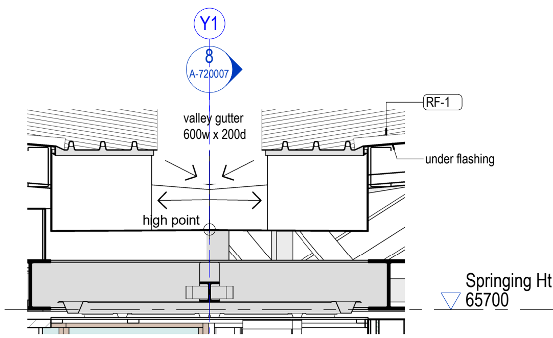
9 Valley Gutter Discharge Elevation 1:20
