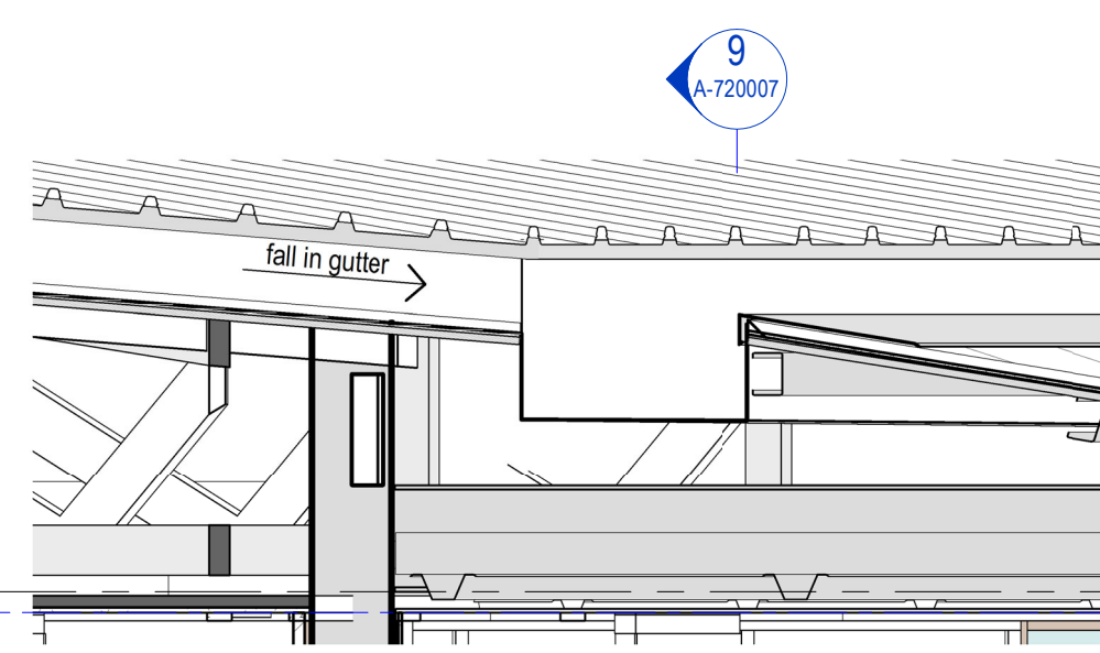
8 Valley Gutter Discharge 1:20
